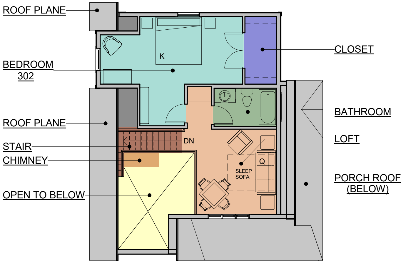
Dock Master's Cottage - Second Floor
