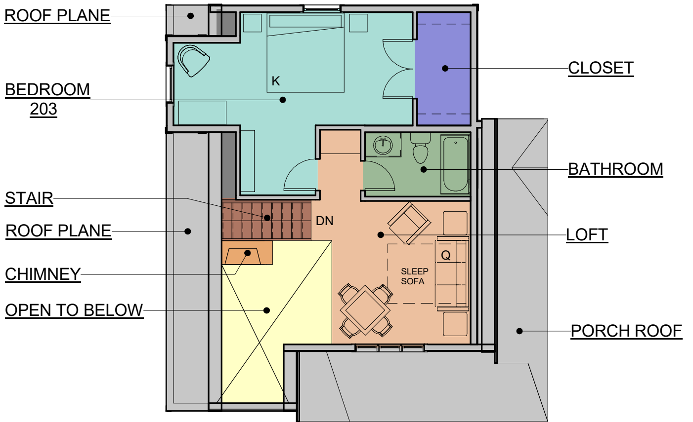
Writer's Cottage - Second Floor
